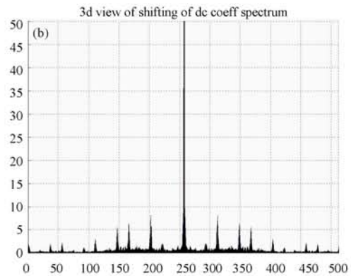
Fig. 8 (a, b): Central spatial frequency spectrum of original flawless sample used for comparison in the detection of double yarn defect
