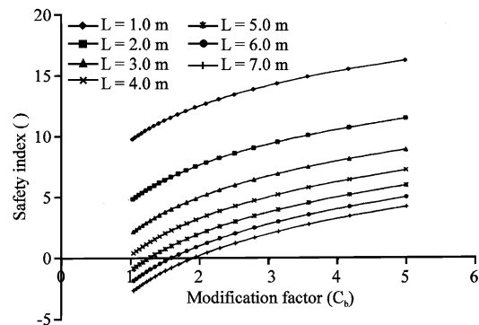
Fig. 2: Safety levels for 152×152 mm×23 kg m -1 UC
