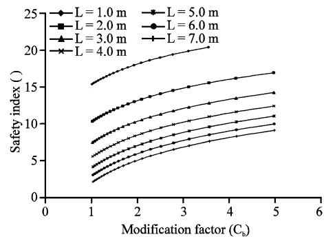
Fig. 16: Safety levels for 305×305 mm ×118 kg m -1 UC
