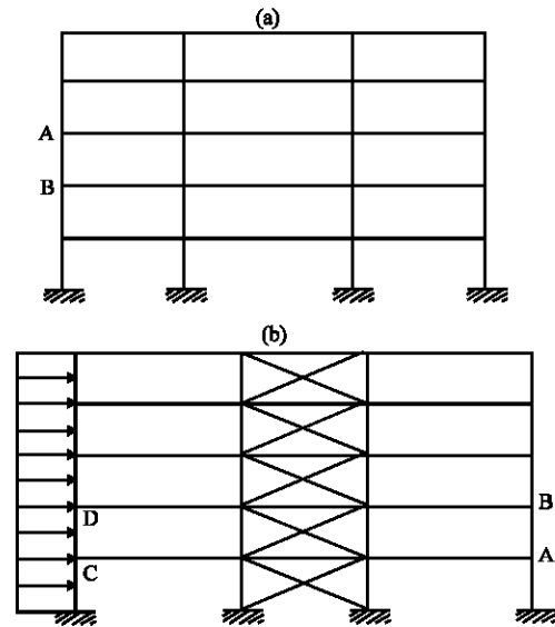
Fig. 1: Frames with and without sideways (a) un-braced frame (b) braced frame
