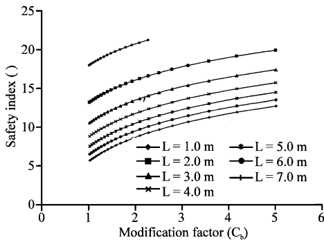
Fig. 28: Safety levels for 356×406 mm ×340 kg m -1 UC
