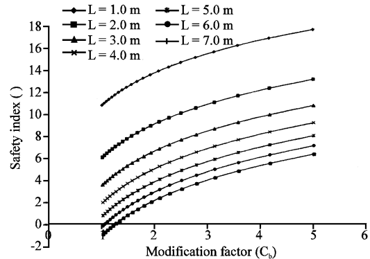
Fig. 4: Safety levels for 152×152 mm×37 kg m -1 UC
