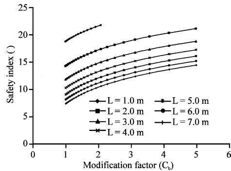
Fig. 31: Safety levels for 356×406 mm ×551 kg m -1 UC
