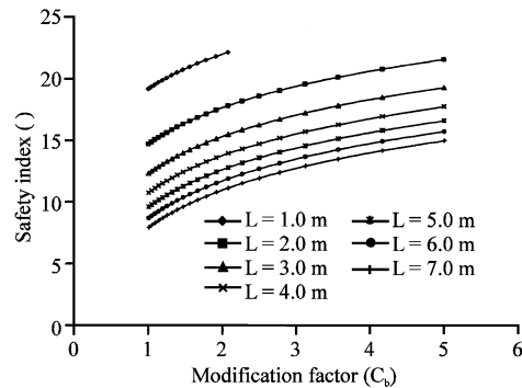
Fig. 32: Safety levels for 356×406 mm ×634 kg m -1 UC
