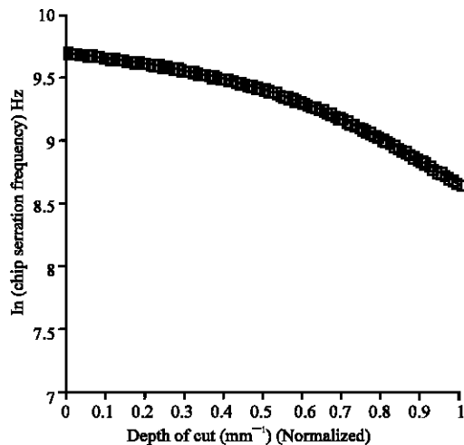
Fig. 7: Effect of depth of cut effect on chip serration predicted by ANN
