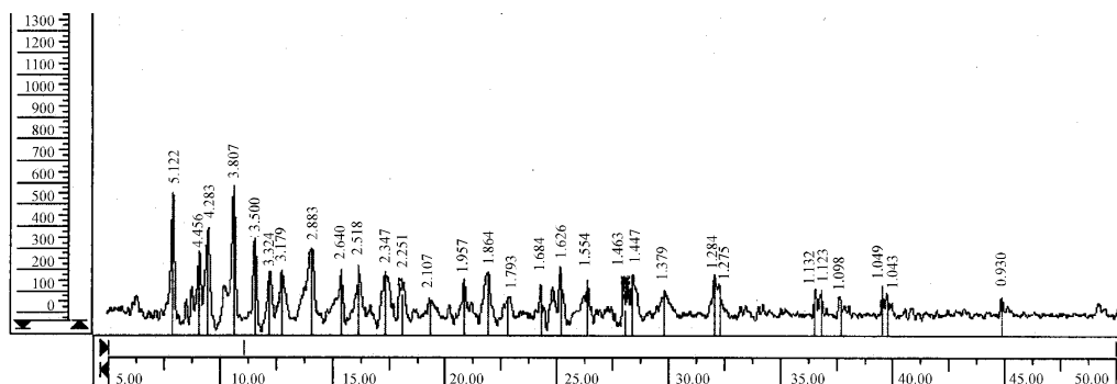
Fig. 4: The XRD diffraction patterns of MnCl_2 in the absent of applied magnetic field
