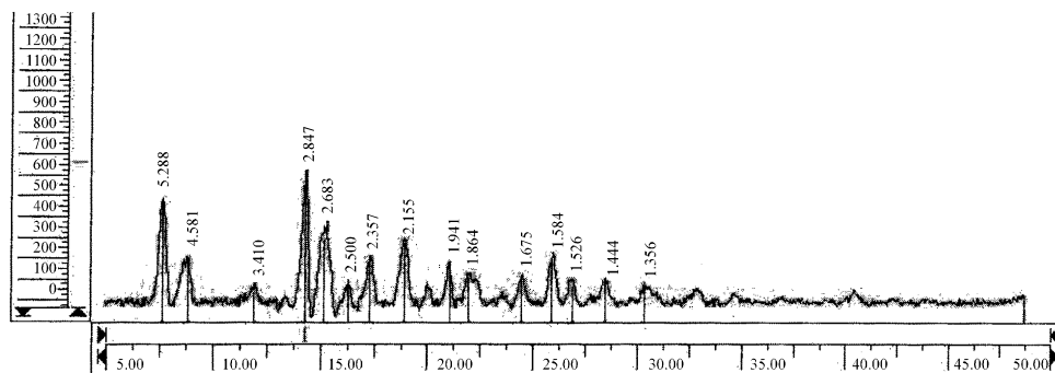
Fig. 2: The XRD diffraction patterns of \text{CoCl}_2 in the absent of applied magnetic field
