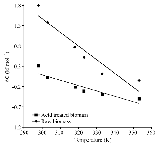
Fig. 8: The free energy change versus temperature for the sorption of Mn (II) ions
