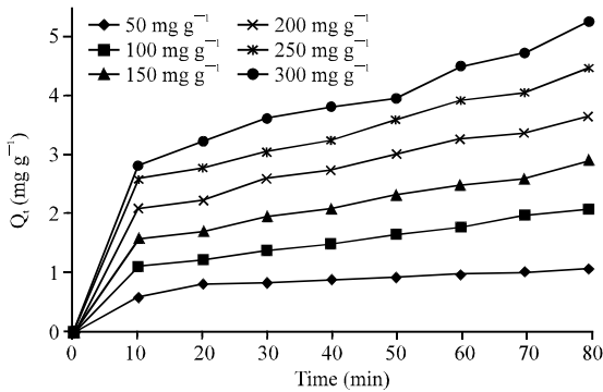
Fig. 1: The variation of adsorption capacity with biosorption time at various concentrations of Mn (II) ions at 25°C (pH 3, W = 1 g raw biomass)
