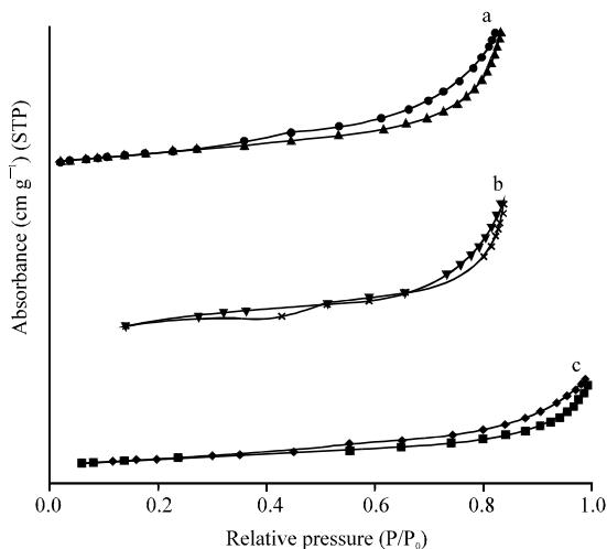
Fig. 2: N 2 adsorption isotherm of; a) Natural; b) Ti-intercalated and c) Ti-pillared bentonite
