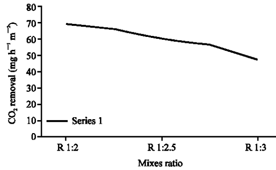
Fig. 3: Influence of TiO 2 and local material on carbon dioxides photo degradation under UV light after 1 week
