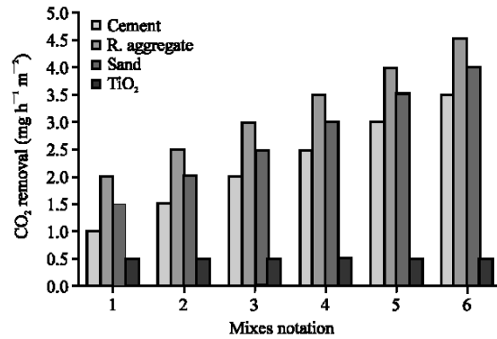
Fig. 4: Influence of TiO 2 and cement/aggregate ratio on carbon dioxides photo degradation under UV light after 2 weeks
