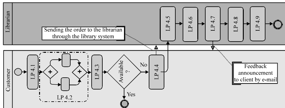
Fig. 3: Sequence flow diagram of the library process 4
