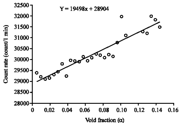
Fig. 5: Experimental results of count rate versus the void fraction ( \alpha ) in case of Pyrex tube filled with crude oil and plastic tubes filled with water
