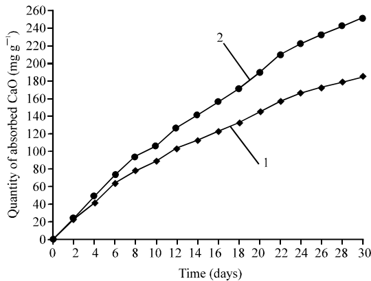
Fig. 2: Kinetic curves of the absorption of calcium oxide with; 1: fine and 2: ultrafine perlite
