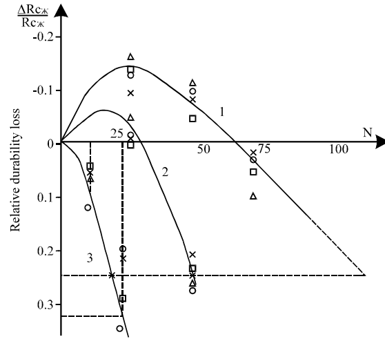
Fig. 2: Ceramsite concrete frost resistance dependence on test temperature; 1: t_1 = -15^\circ\text{C} , \Delta R_{cж}/R_{cж} = 9.88 \cdot 10^{-5} N^2 ; 2: t_1 = -34^\circ\text{C} , \Delta R_{cж}/R_{cж} = 2.48 \cdot 10^{-4} N^2 - 7.4 \cdot 10^{-3} N ; 3: t_1 = -55^\circ\text{C} , \Delta R_{cж}/R_{cж} = 4.17 \cdot 10^{-4} N^2 + 5.84 \cdot 10^{-3} N
