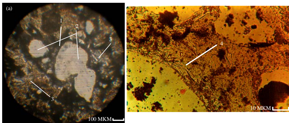
Fig. 1: Photomicrographs of fragmented microreinforced porous structure (T firing -1050°C); a) composition (4 gs); b) composition (4 k): 1: fragment of the structure; 2: pores; 3: interfragmentary space crystallization; 4: treads microreinforced with plated needles
