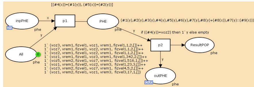
Fig. 2: Hierarchical model of POP synthesis
