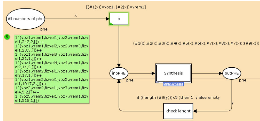
Fig. 2: Hierarchical model of POP synthesis
