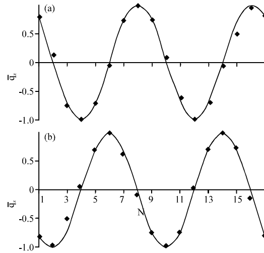
Fig. 4: Scatter of displacements of peripheral points of blades for vibrations of the initial model under paired modes with m = 2 ; —: Computation, •: experiment
