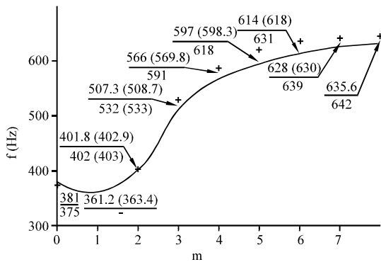
Fig. 3: The spectrum of eigen frequencies of an initial design: -: Computation, +: experiment; f_m^{(1)} ( f_m^{(2)}/f_{me}^{(1)} ( f_{me}^{(2)} ) the eigen frequencies of paired modes defined by computation ( f_m^{(1)} , f_m^{(2)} ) and experimentally ( f_{me}^{(1)} , f_{me}^{(2)} )
