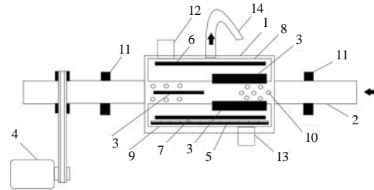
Fig. 2: Scheme of construction unit of grain processing part
