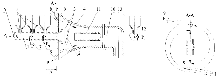
Fig. 1: Counterflow pneumatic mixer: 1: feed pipe; 2: closed end; 3: outlets; 4: case; 5: input nozzles; 6, 7, 12: air nozzles; 8: large end; 9: inclined air nozzles; 10: pipe branch; 11: radial holes
