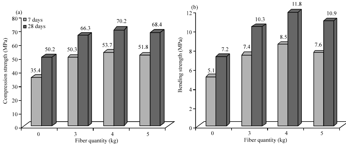
Fig. 3: Results of experimental investigations of fine-grain fiber-reinforced concrete; a) compression strength; b) bending strength
