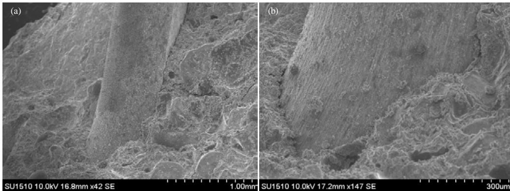
Fig. 4: Microstructure of a contact zone “set cement polypropylene fiber”; a) with use of VNV-100; b) with use of Cem I 42.5N
