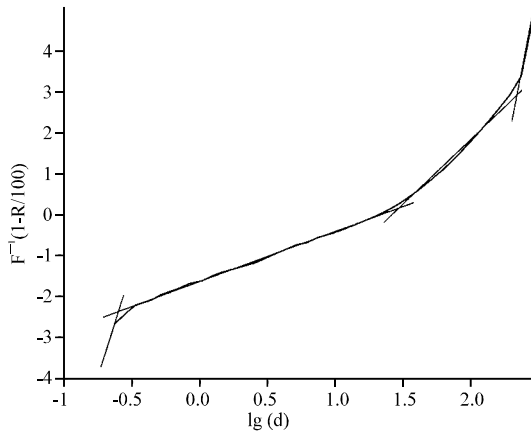
Fig. 6: Granulometric composition of cement on log-probability grid d-F^{-1}(1-R/100)
