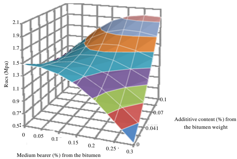
Fig. 2. : Dependences of the ultimate asphalt concrete strength at 50°C on the amount of medium-bearer and the amount of FCM. (Additive content, % from the bitumen weight: Medium-bearer content, % from bitumen weight)
