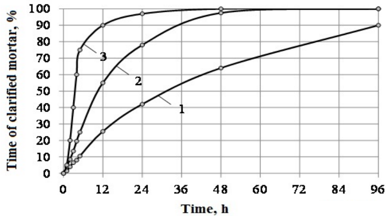
Fig. 1: Curve of particles sedimentation
