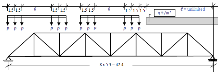
Fig. 3: Identification of members load
