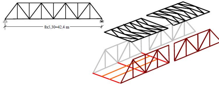
Fig. 1: Free body sketch of the BH 1549
