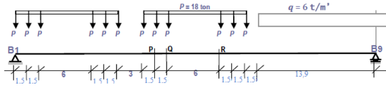
Fig. 4: Identification of members load is shown in
