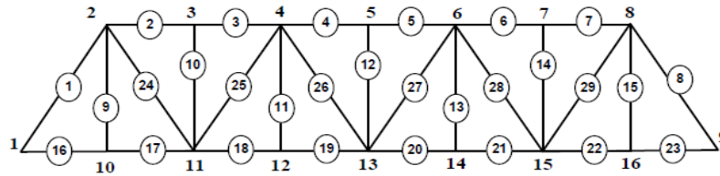
Fig. 2: Numbered joints and members of the BH 1549 steel-truss railway bridge model
