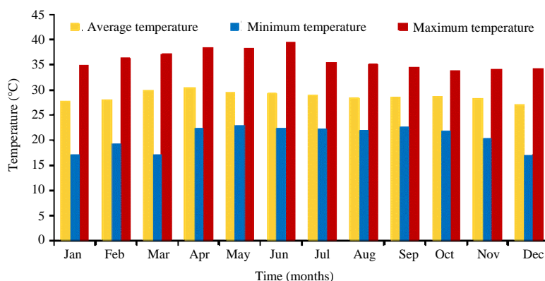
Fig. 3: Average, maximum and minimum temperature in the study area from 1984-2015
