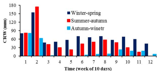
Fig. 7: Crop water requirements for three crops
