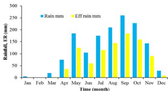
Fig. 6: Simulation results of effective rainfall and rainfall with time
