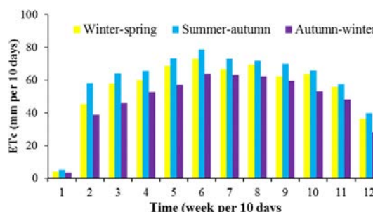
Fig. 5: Calculation results of ET C from three rice crops
