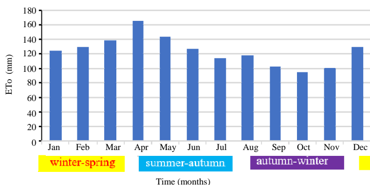
Fig. 4: Simulation results of ETO with time
