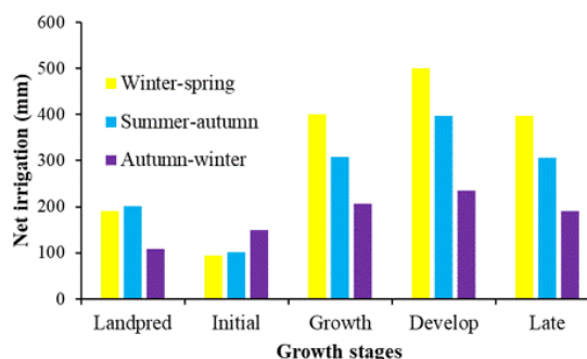
Fig. 8: Irrigation requirement for growth stages of the three rice crops
