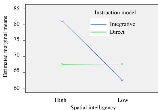
Fig. 2: Graphics of interaction between instruction model and spatial intelligency towards mathematics learning outcome after being controlled by the prior competence
