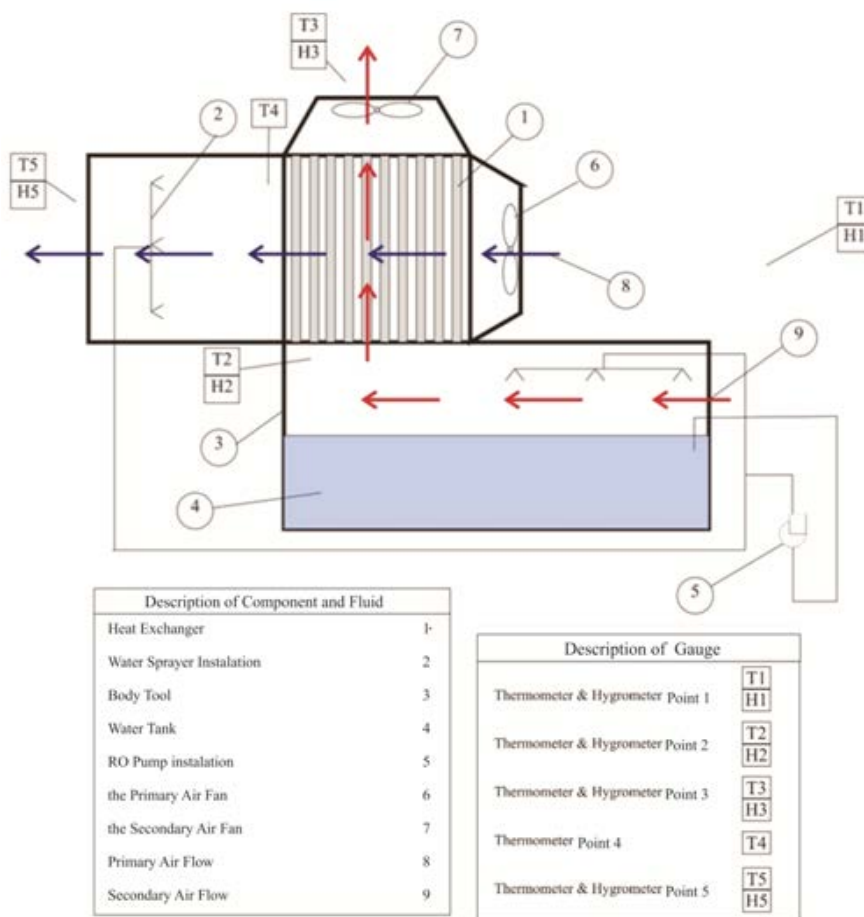
Fig. 3: Schematic and testing point two level indirect-direct evaporative cooler
