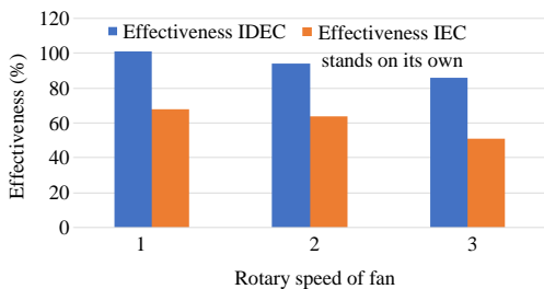
Fig. 6: Comparison of IDEC effectiveness
