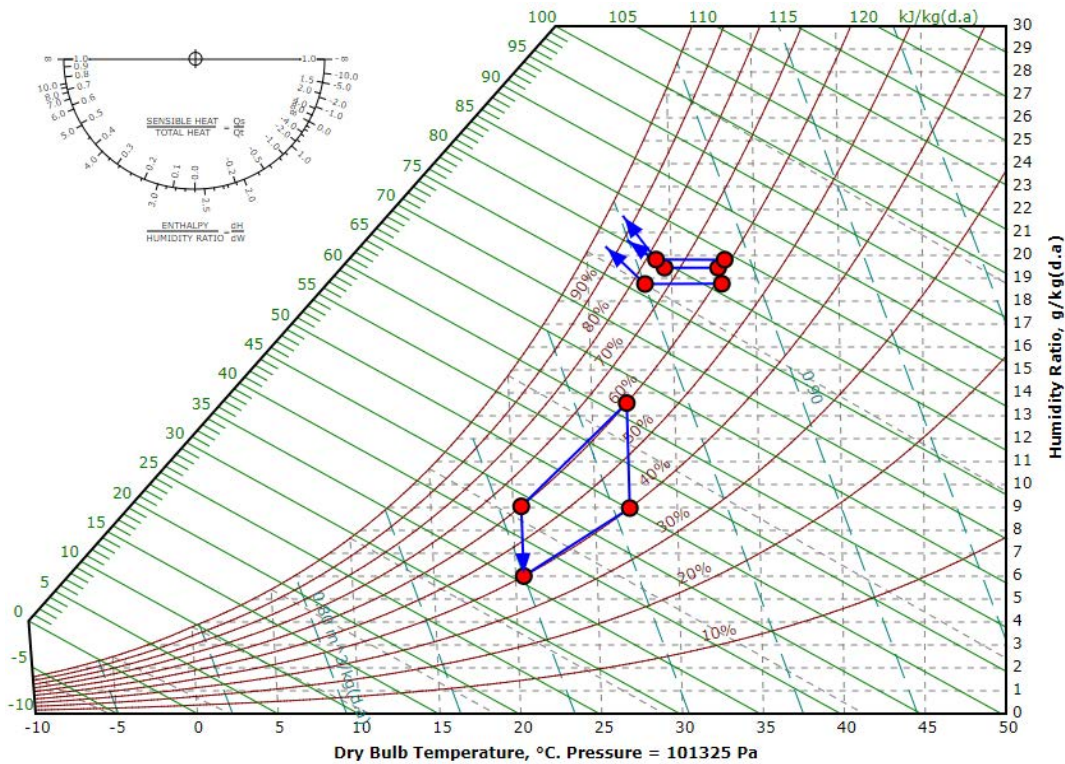
Fig. 5: The test results are compared with the standard comfortable air condition SNI in the psychometrics diagram
