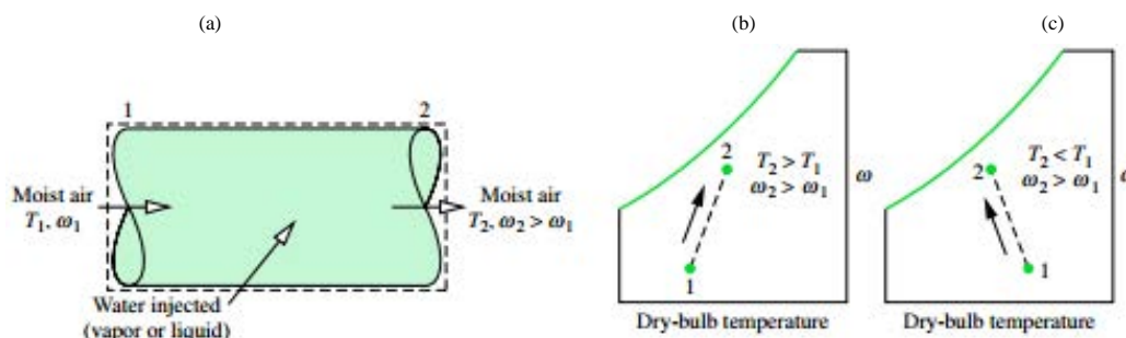
Fig. 1(a-c): Humidification: a) Control volume; b) Steam injected and c) Liquid injected
