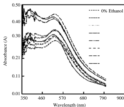
Fig. 14: UV-visible spectra of gold nanoparticles for 0% ethanol/water mixture for different concentration of NDT
