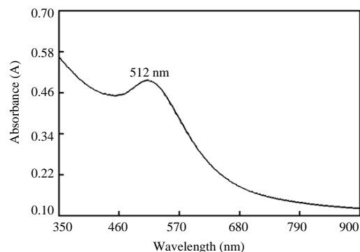
Fig. 1: UV-visible spectrum of gold nanoparticles used as seeds
