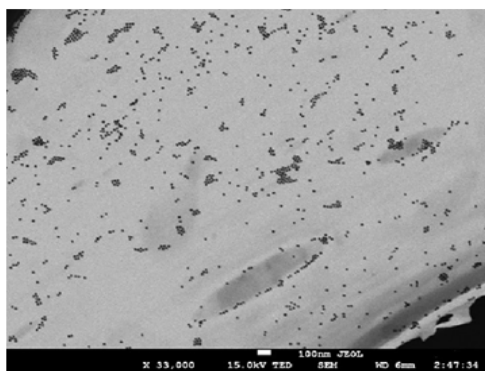
Fig. 9: FESEM micrograph of citrate stabilized gold nanoparticles
