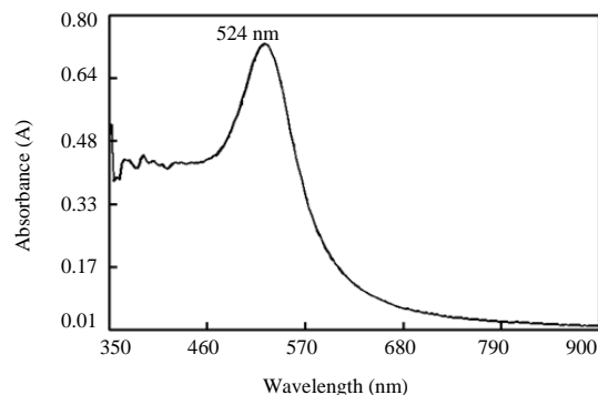
Fig. 2: UV-visible spectrum of gold nanoparticles (A)
