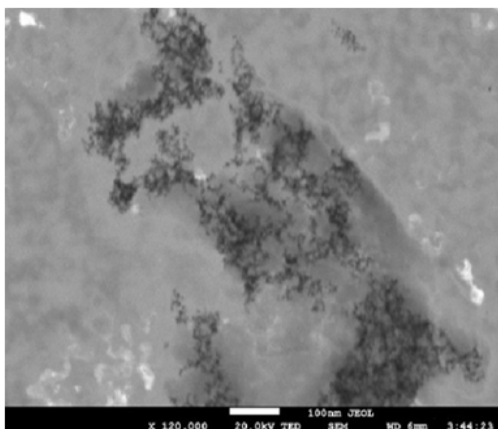
Fig. 12: TEM micrograph of gold nanoparticles
