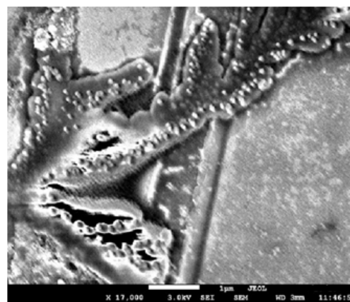
Fig. 11: FESEM micrograph of gold nanoparticles synthesized by borohydride reduction method
