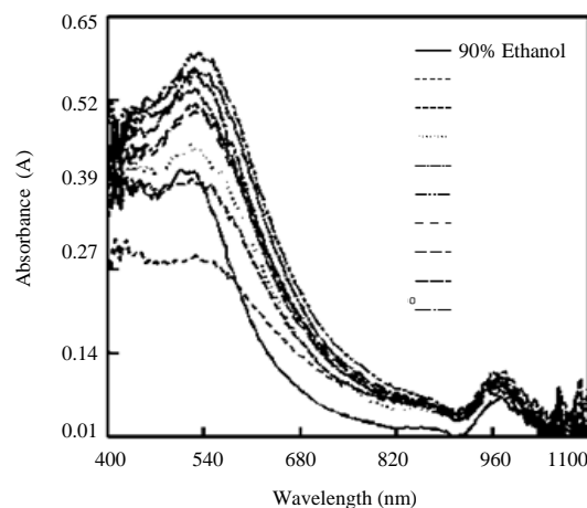
Fig. 15: UV-visible spectra of gold nanoparticles 90% ethanol/water mixture for different concentration of NDT
