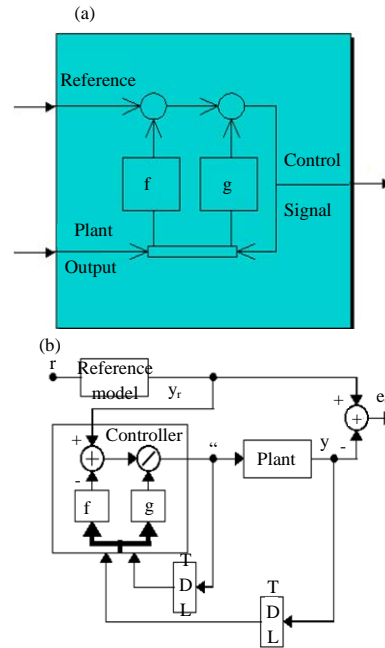
Fig. 8: Block controller of NARMA
