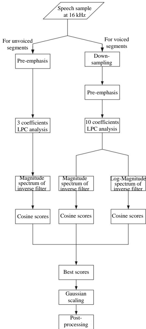
Fig. 6: Flowchart of proposed scheme for automatic segmentation of speech based on FICV [24]
