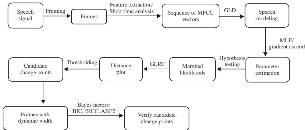
Fig. 4: Block diagram of the proposed TI segmentation system [18]
