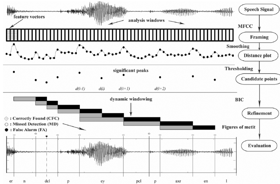
Fig. 5: Block diagram of DISTBIC phonemic segmentation algorithm [32]
