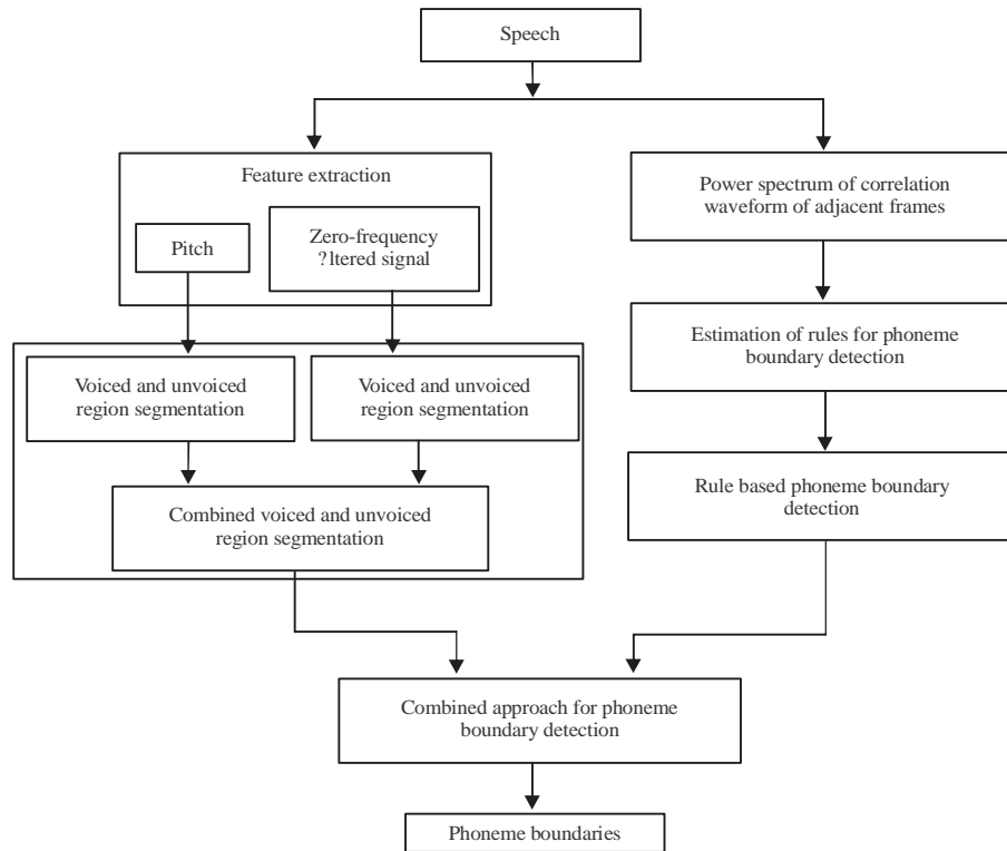
Fig. 7: Phoneme boundary detection: a rule based approach [19]
