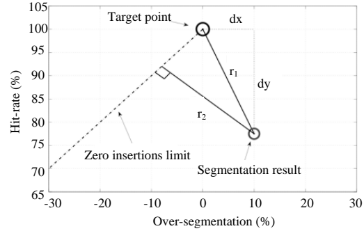
Fig. 2: Calculating R-measure [18]
