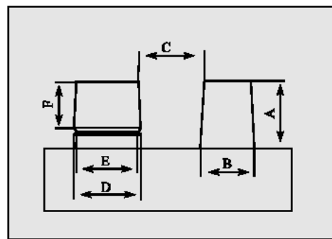
Fig. 2: Height of die without undercut (A), Die diameter without undercut (B), Distance between two die from each other (C), Die diameter below the undercut (D), Inside diameter of undercut (E), Height of above the undercut (F)
