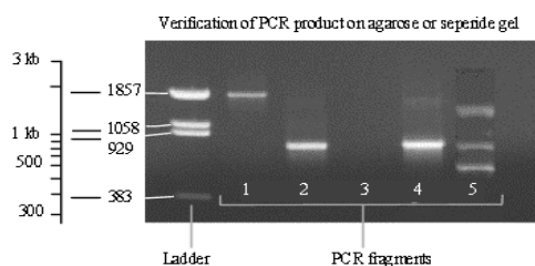
Fig. 2: Verification of the PCR product on gel
