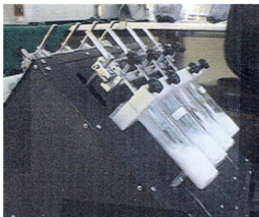
Fig. 2: V8 cross brushing machine
