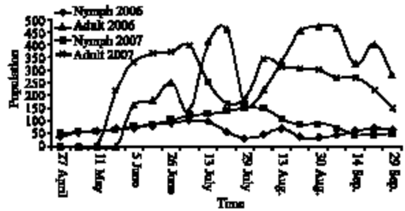
Fig. 6: Population fluctuation of Philaenus spumarius (L.) in Mashhad region in 2006-2007
