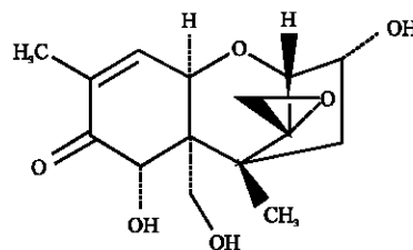
Fig. 1: Deoxynivalenol(12,13-epoxy-3 \alpha ,7 \alpha ,15-trihydroxy-trichothec-9-ene-8-one)
