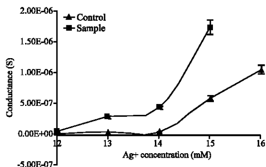
Fig. 2: Consequence of Ag ion concentration on conductance. Experimental condition: the hemin concentration 250 \mu\text{M} in DMF and RNA concentration 10-12 M, reaction time 5 min
