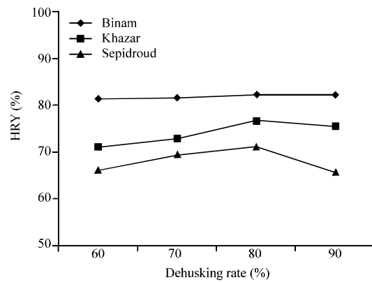
Fig. 4: Effect of dehusking rate on the HRY of the tested varieties
