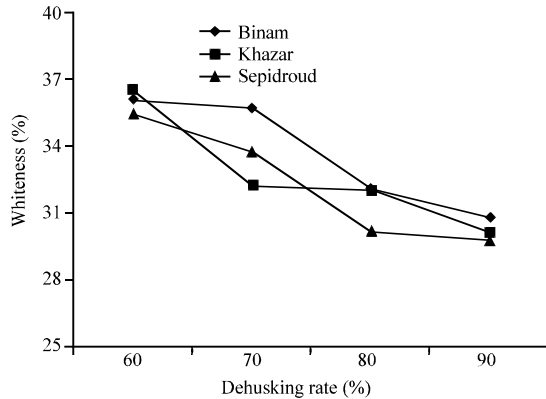
Fig. 6: Effect of dehusking rate on the rice whiteness of different varieties
