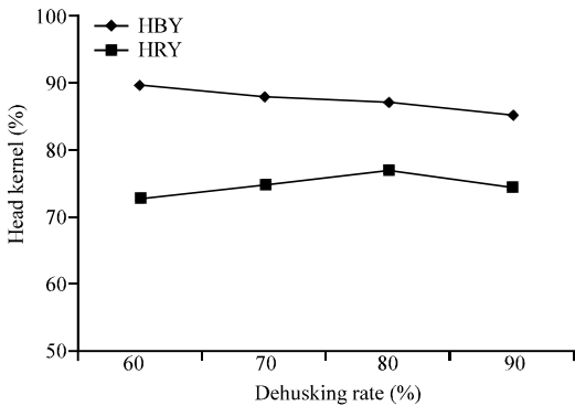
Fig. 3: Independent effect of dehusking rate on the HBY and HRY
