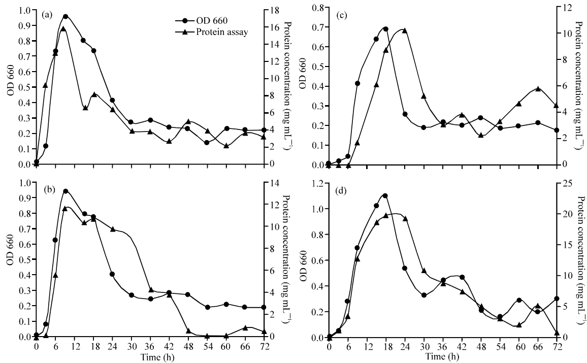
Fig. 1: Growth curves of P. aeruginosa PDMZnCd2003 in nutrient broth (control) and nutrient broth supplemented with Zn and/or Cd, monitored by turbidimetric method and protein assay; a) Nutrient Broth (NB); b) NB with Zn; c) NB with Cd and d) NB with Zn plus Cd
