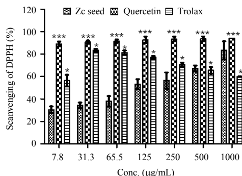
Fig. 1: Antioxidant activities of Zizyphus spina-christi crude extracts (2 mg mL -1 ), quercetin and trolox (500 \mu\text{g mL}^{-1} ). Free radical scavenging inhibitory activities was measured using DPPH assay. Absorbance was taken at 517 nm with quercetin and trolox as standards. ***p<0.0001 represented significantly different values from standards and tested plants. The values represent mean \pm SD from three independent experiments
