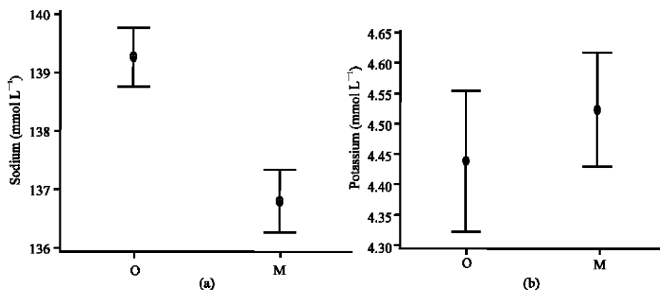
Fig. 5: Interval plots for (A): Sodium and (B): Potassium (O: Olympus AU640 and M: Microlyte 6.0)
