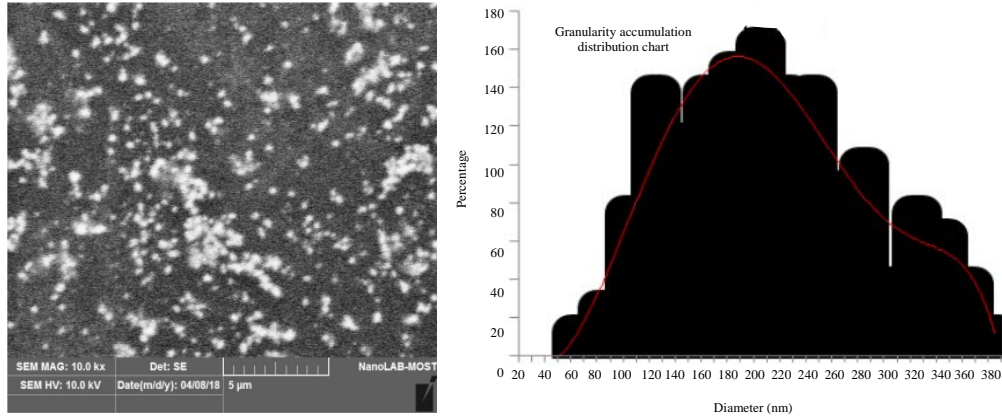
Fig. 2: SEM for 0.531 μM of AuNPs
