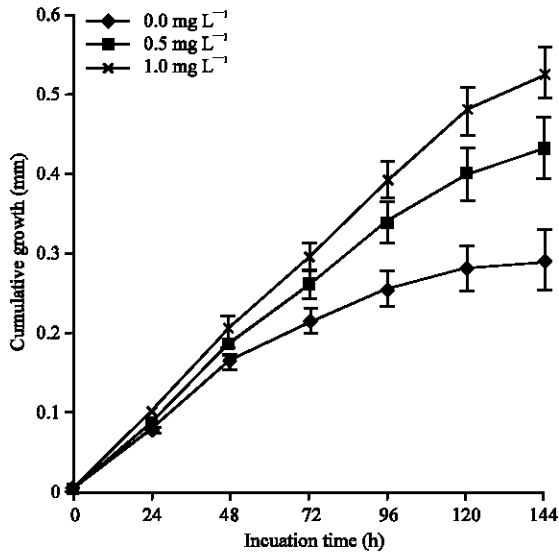
Fig. 2: The effect of different concentrations of biotin on the cumulative growth of isolated secondary wool follicles in vitro . Results expressed as least square means±S.E.M. of increase in cumulative growth of total (viable and quiescent) follicles. Measurements were made on 90-100 follicles per treatment initially isolated from three sheep (30-35 follicles from each sheep for each concentration)
