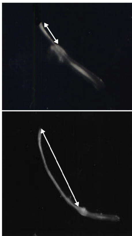
Fig. 1: Light micrograph showing increase in wool follicles length (arrow) with time culture (a) after 24h in culture and (b) after 96 h incubation in Williams' E (s) medium (×25)
