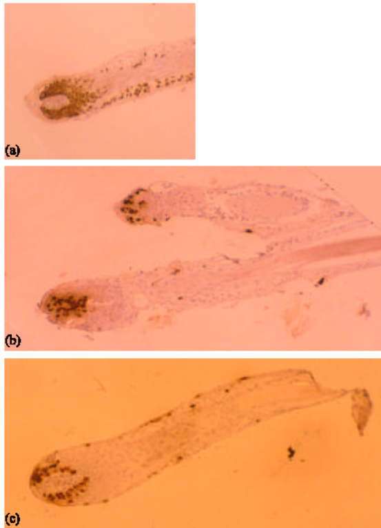
Fig. 4: The pattern of BrdU incorporation following DNA synthesis in wool follicles immunostained by the biotin-streptavidin method; longitudinal section of freshly isolated follicles, showing BrdU uptake by matrix cells adjacent to dermal papilla; (b) hair follicle maintained in biotin-free media for 72 h, with apparently reduced but similar pattern of BrdU incorporation in the matrix as in freshly isolated follicles, (the cells of dermal papilla became disorganised) and (c) hair follicle maintained in biotin-supplemented media for 72 h with BrdU incorporation showing a similar pattern of DNA synthesis ( \times 200 )
