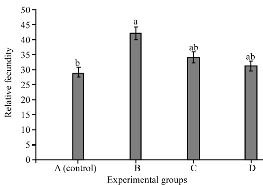
Fig. 2: Relative fecundity of different experimental groups of Xiphophorus helleri . Means with the same letters are not significantly different ( p > 0.05 ). Data are expressed as mean±SE
