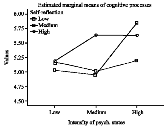
Fig. 1: Influence of the mental states intensity on the cognitive processes productivity depending on the level indices of reflexivity
