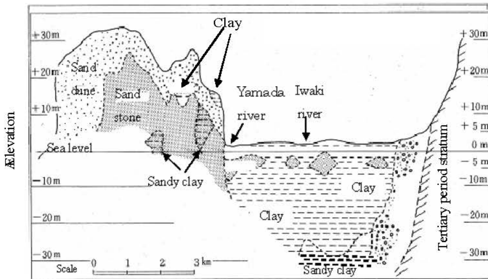
Fig. 2: Cross section of the study area showing geology (Byoubusan Land Improvement District, 1991)
