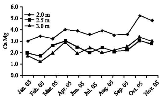
Fig. 10: Ratio in Ca an Mg in groundwater at different depth
