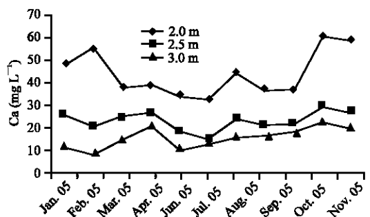
Fig. 6: Calcium concentration in groundwater at different depth
