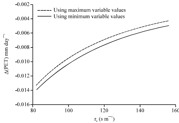
Fig. 2: Response of PET estimates to unit step increases (1 s m -1 ) over the range of possible values in Botswana for the parameter r_a in the Penman-Monteith equation using maximum and minimum values of the input variables with r_s = 70 \text{ s m}^{-1}
