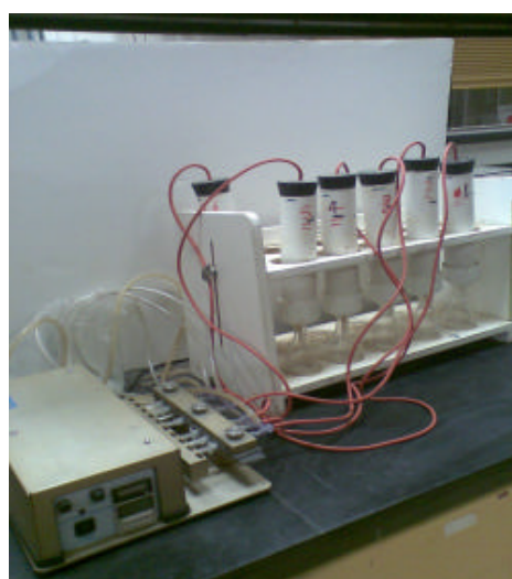
Fig. 1: A picture of the column experiment for nitrate leaching
