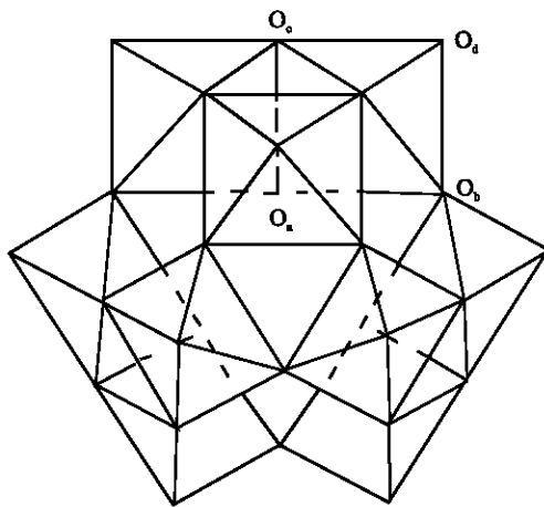
Fig. 1: The structure of Keggin type heteropoly anion
