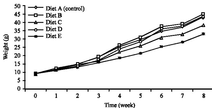
Fig. 1: Growth performance of juvenile Clarias gariepinus fed Ipomoea aquatica diet inclusion
