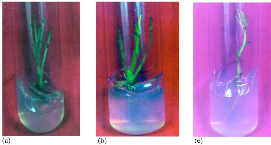
Fig. 1: (a) Effect of BA and Kin (b) Effect of Auxin and (c) Effect of combination on shoot and root formation
