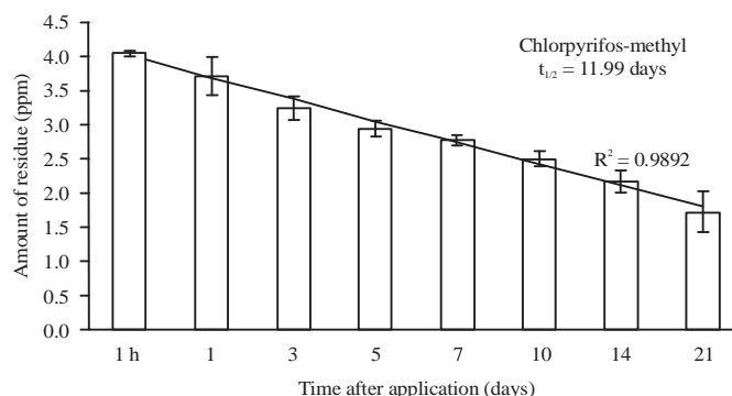
Fig. 1: Disappearance pattern and half-time values of chlorpyrifos-methyl after 1 h, 3, 5, 7, 10, 14 and 21 days of last spray application, t_{1/2} = \ln_2/K = 0.693/K , K = 1/t \times \ln a/m , where, K is apparent rate constant, t is time in days, m is residue at x time and a is initial residue
