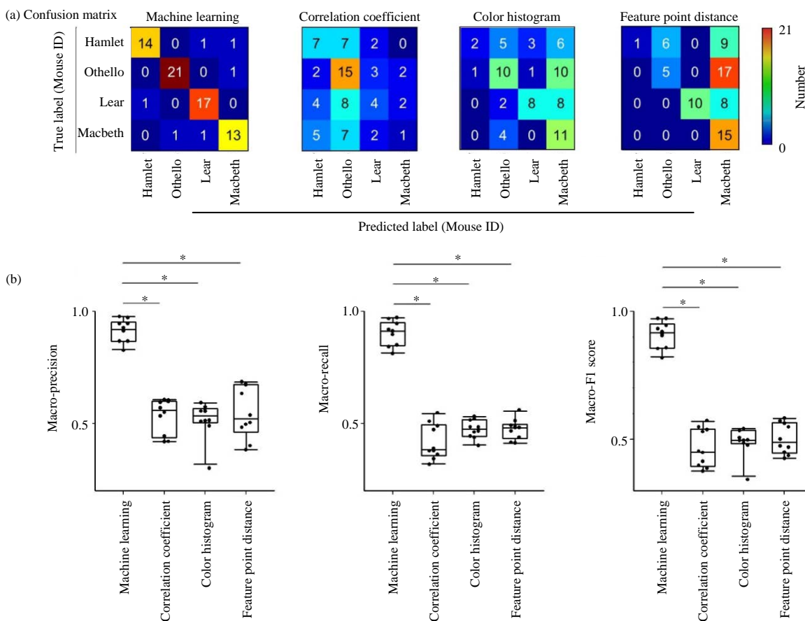
Fig. 3(a-b): Comparison of the individual identification performance between our algorithm and others
