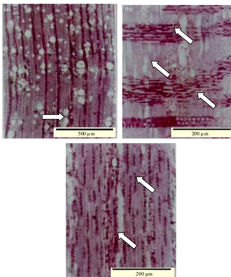
Fig. 2(a-c): (a) Cinnamomum burmannii blume samples obtained from the solok, West sumatera (40 \times magnification). Diffuse-porosity at transverse section, (b) Radial section of procumbent body ray cells (arrows showed one row of upright or square marginal cells and some rays with procumbent, square and upright cells mixed, oil cells associated with axial parenchyma) and (c) (-1) 2 seriate rays at tangential section
