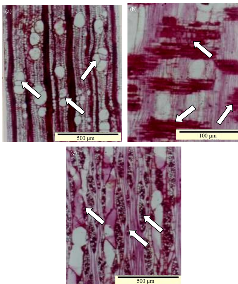
Fig. 5(a-c): Cinnamomum coriaceum wood samples obtained from the maros, south Sulawesi/Celebes (40×magnification), (a) Transverse section: Multiple vessels of 2-3(-4-6) and clusters, oil cells present among the fibres, (b) Radial section: Body ray cells procumbent with 1-3 rows of upright and square marginal cells, all ray cells procumbent, some rays with procumbent, square and upright cells mixed and (c) Tangential section: (-1-2)-3-5 seriate rays and simple perforation plate
