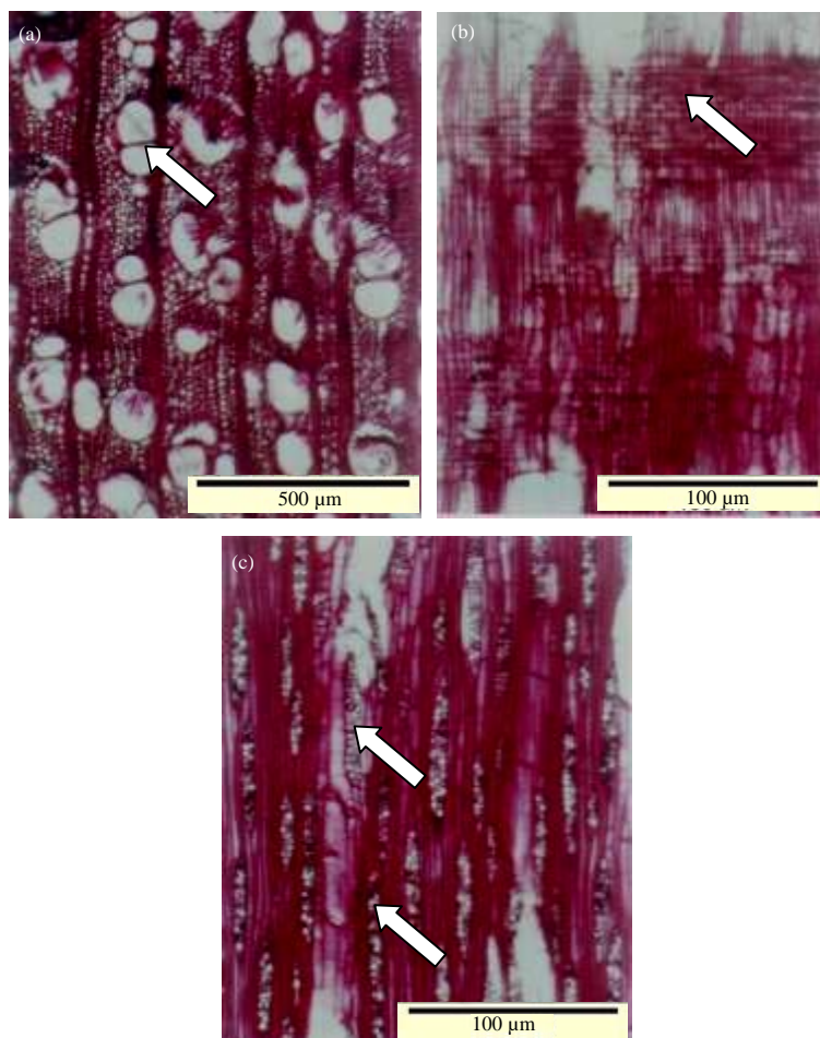
Fig. 4(a-c): Cinnamomum zeylanicum blume samples obtained from the kerinci, jambi (40×magnification), (a) Transverse section: Multiples vessel of 2, (b) Radial section: All ray cells upright and square and (c) Tangential section: 2-3 seriate rays
