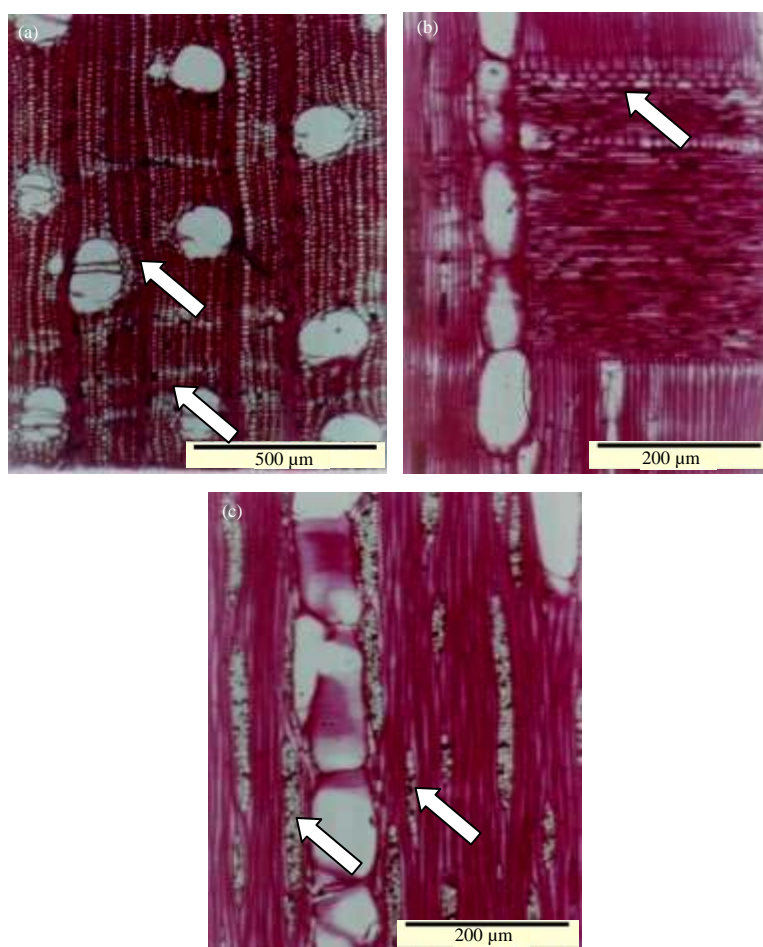
Fig. 6(a-c): Cryptocarya aromatica kostermans samples obtained from collection of the xylarium bogoriense 1915 bogor, Indonesia (40×magnification), (a) Transverse section: Axial parenchyma vasicentric and axial parenchyma bands 3-4 cells wide, (b) Radial section: Body ray cells procumbent with 3 rows of upright and square marginal cells and (c) Tangential section: (-2)-5 seriate rays
