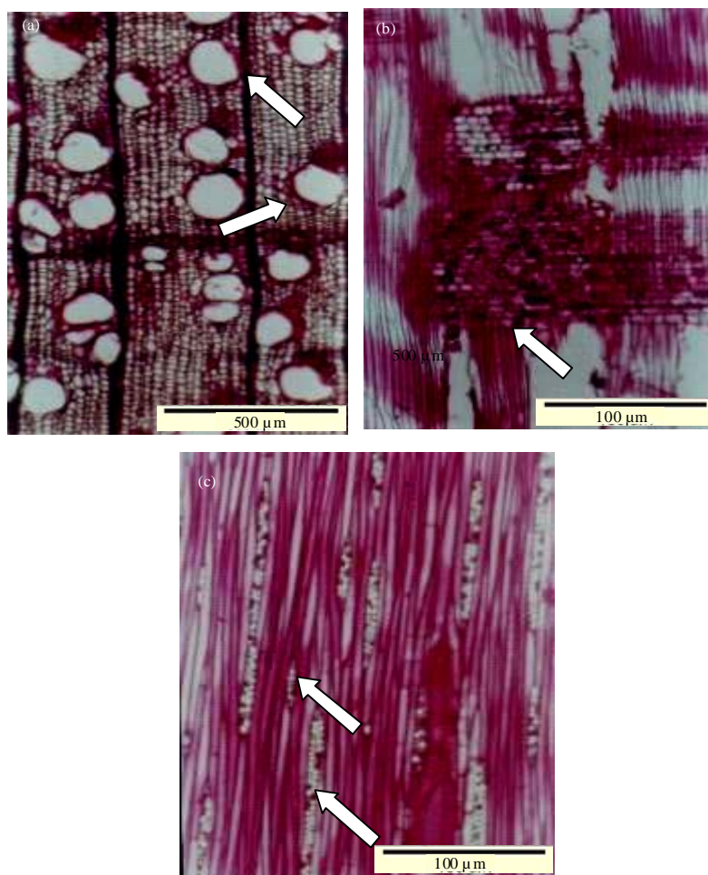
Fig. 3(a-c): Cinnamomum xanthoneureum Blume samples obtained from the Donggala, Central Sulawesi/Celebes (40×magnification), (a) Transverse section: Parenchyma unilateral paratracheal and vasicentric, (b) Radial section: Procumbent body ray cells with one row of upright or square marginal cells and (c) Tangential section: 1-2 seriate rays
