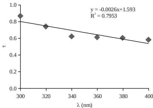
Fig. 3: Total atmospheric extinction value at UV radiation wavelength
