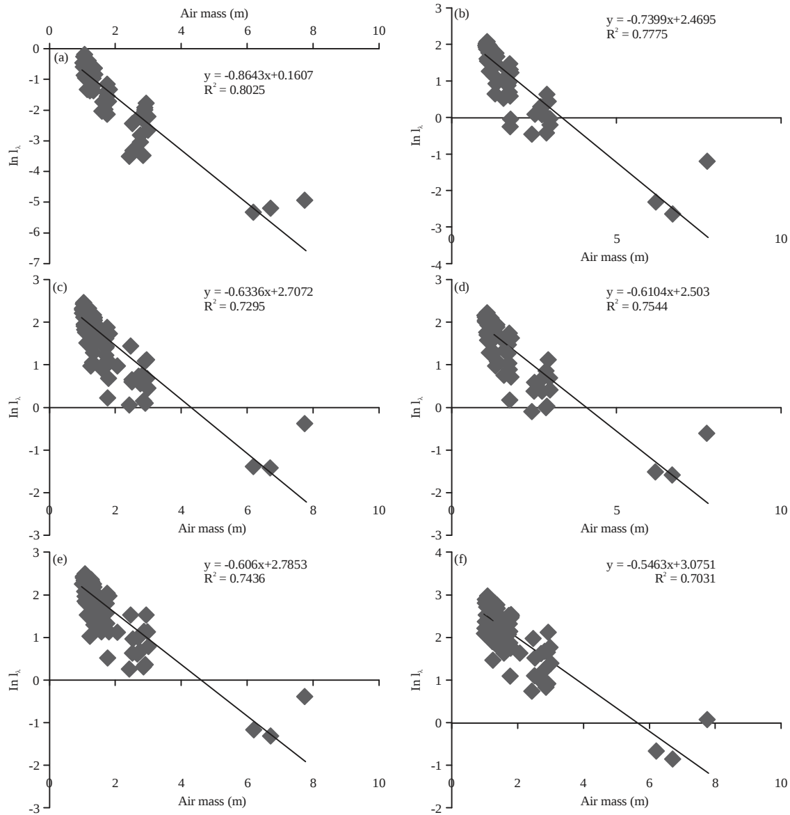
Fig. 2(a-f): Example for Langley plot for UV radiation and respective liner functions obtained by the least square from January-March, 2014, (a) 300 nm, (b) 320 nm, (c) 340 nm, (d) 360 nm, (e) 380 nm and (f) 400 nm
