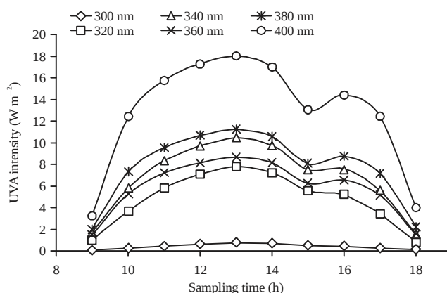
Fig. 1: Example of calculated solar irradiance in the ultraviolet between 300 and 400 nm for January-March, 2014 at Bangi
