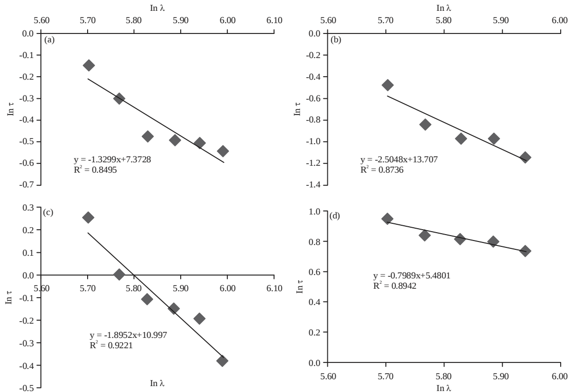
Fig.4(a-d): Liner regression equation for 12 months in 2014, each three months present on one linear, (a) January-March, (b) April-June, (c) July-September and (d) October-December
